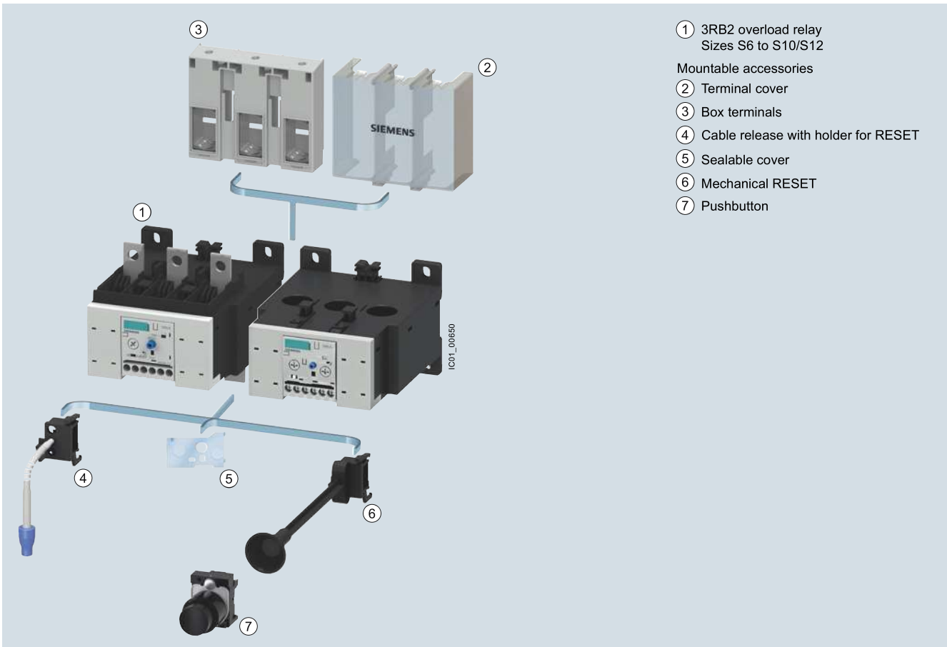
Mountable accessories for 3RB2 electronic overload relays (sizes S6 to S10/S12)
