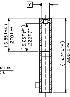
3 TO 32 CKTS. 2 POLARISING BUTTON VERSION
