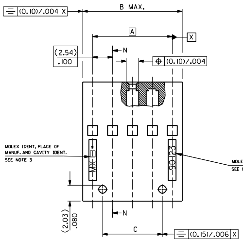
3 TO 32 CKTS. 2 POLARISING BUTTON VERSION
