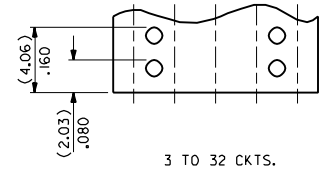
3 TO 32 CKTS. 4 POLARISING BUTTON VERSION
