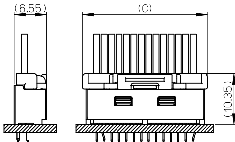
嵌合図 (SCALE 2:1) MATED CONNECTORS (SCALE 2:1)
