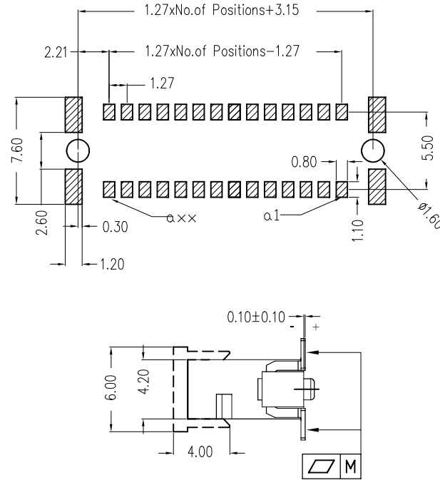
Recommended P.C.B Layout (Top Side) (PCB BOARD TOLERANCE \pm 0.05 )
