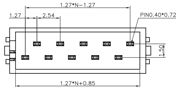
HOUSING
