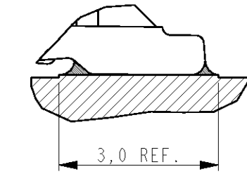
SOLDER DETAIL SCALE 10:1
