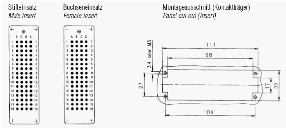
Contact arrangement
