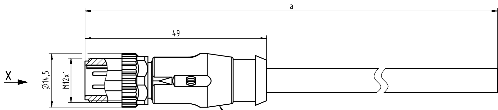
M12 D-coded 4 poles, straight overmolded male connector
