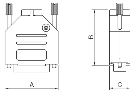
D-Sub-Hood
