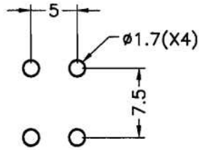
MOUNTING HOLES
