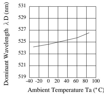
Ambient Temperature vs. Dominant Wavelength
