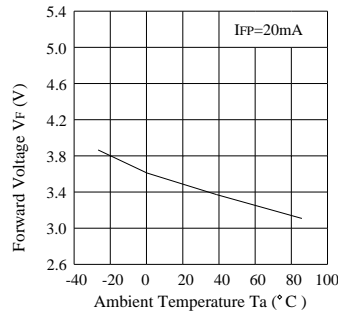
Ambient Temperature vs. Forward Voltage
