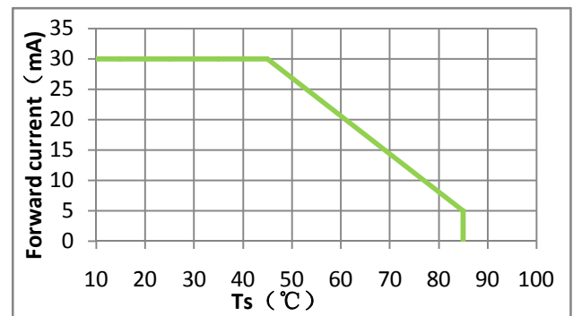
Fig.6- Temperature Vs. Forward Current 引脚温度与正向电流特性曲线
