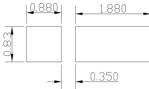
Soldering Patterns
