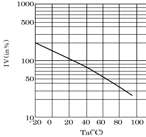
IV-Ta Characteristics
