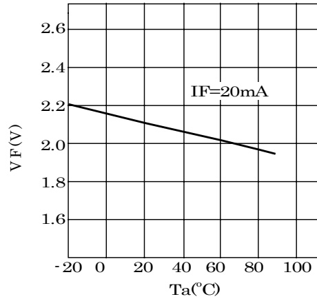
VF-Ta Characteristics
