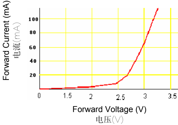
Forward Current vs Forward Voltage 伏安特性曲线
