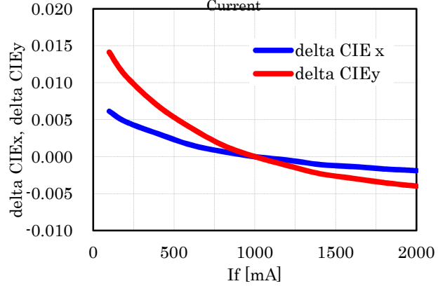
Chromaticity Coordinate Shift by Forward Current
