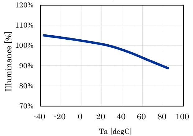
Ta-Intensity Characteristics
