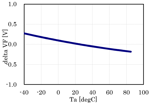
Ta-VF Characteristics
