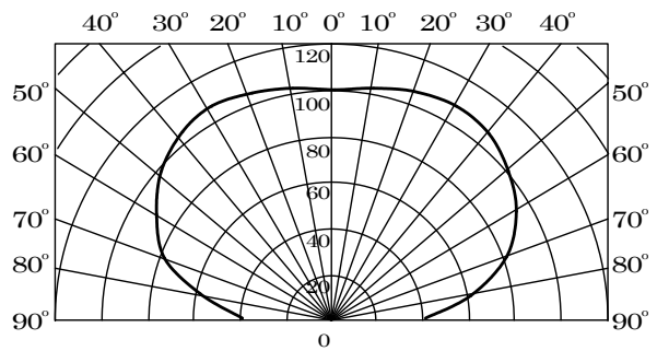
Directive Characteristics
