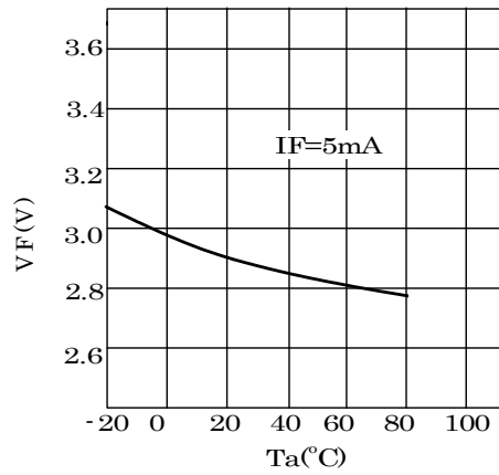
VF-Ta Characteristics
