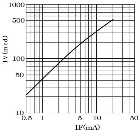
IV-IF Characteristics
