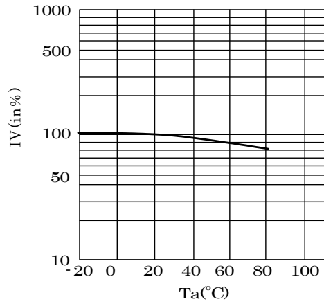
IV-Ta Characteristics
