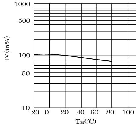
IV-Ta Characteristics
