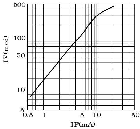
IV-IF Characteristics
