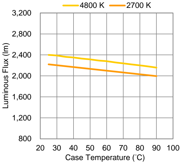
Fig 4. Case Temperature vs. Luminous Flux at 700 mA.
