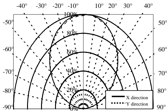
Directive Characteristic
