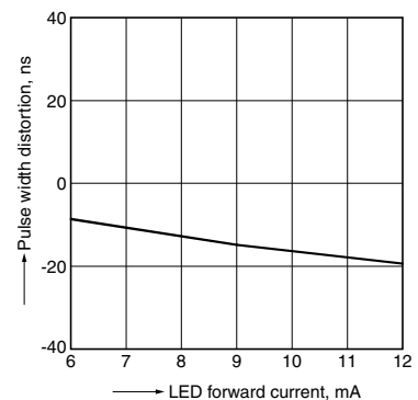
9. Pulse width distortion vs. LED forward current characteristics
