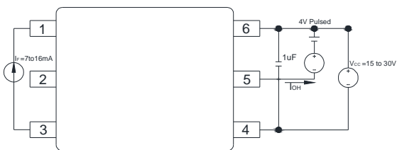
Figure 14 : V_{OH} Test Circuit
