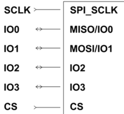
Figure 8. QSPI interface connection
