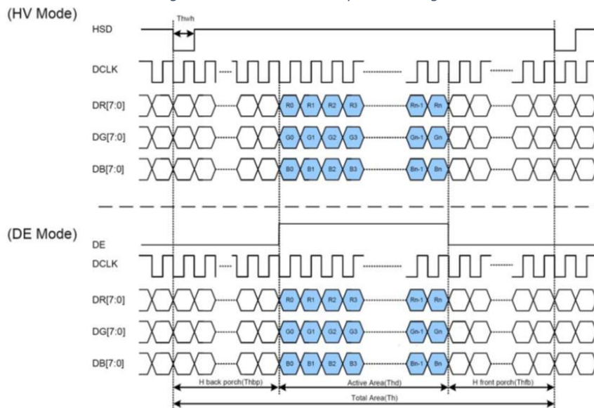
Figure 12. Clock and data input time diagram.
