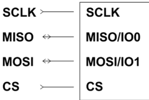
Figure 7. SPI interface connection
