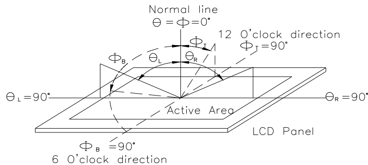
Fig.10.1. Definition of viewing angle
