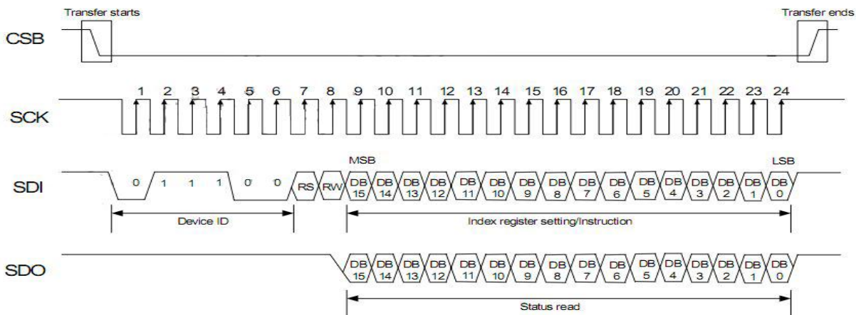
Figure 6 SPI Interface Input Signal Timing
