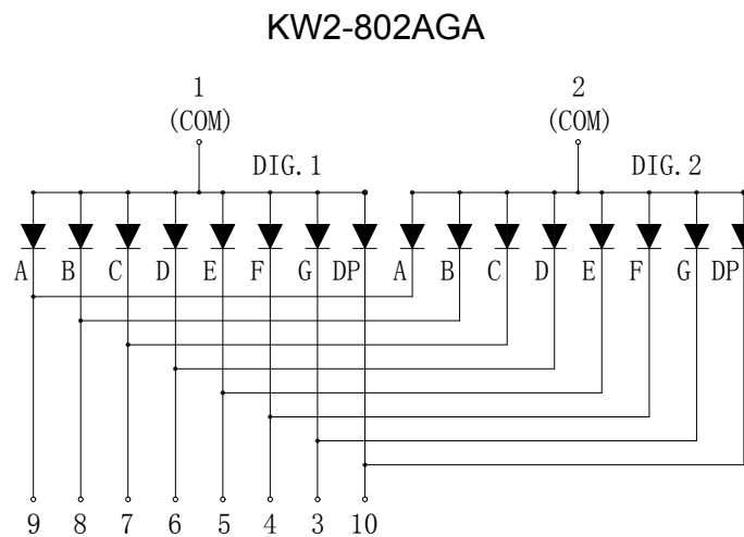
Internal Circuit Diagram (Common Anode)
