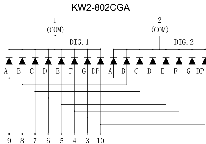
Internal Circuit Diagram (Common Cathode)
