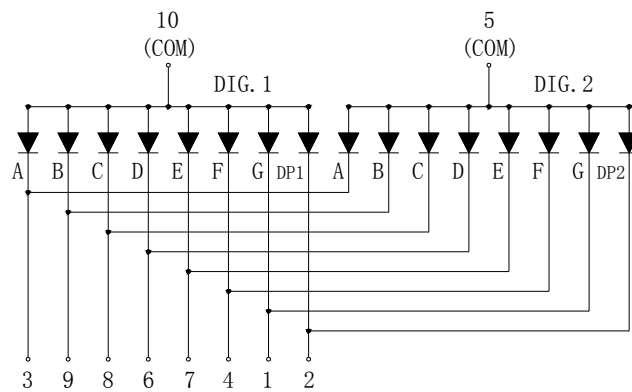
Internal Circuit Diagram (Common Cathode)
