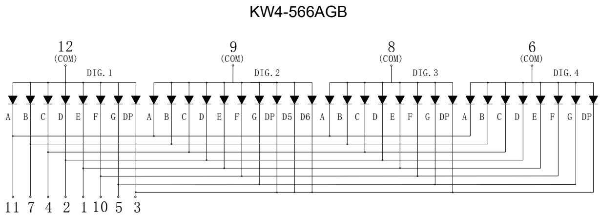
Internal Circuit Diagram (Common Anode)
