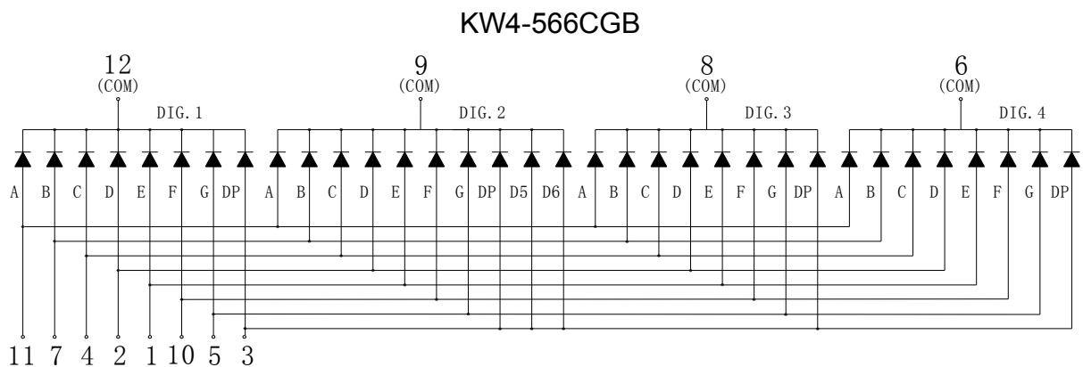
Internal Circuit Diagram (Common Cathode)
