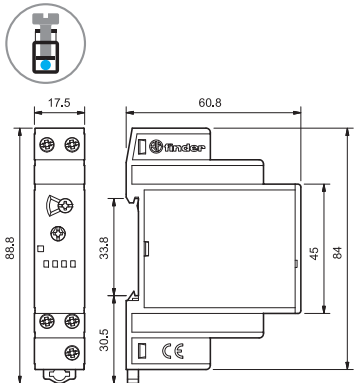
80.61 Screw terminal
