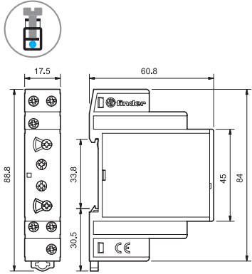
80.91 Screw terminal
