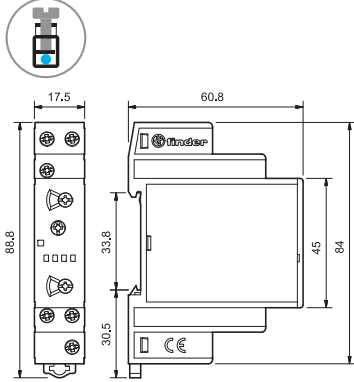
80.01 Screw terminal
