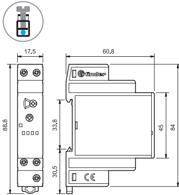
80.21 Screw terminal
