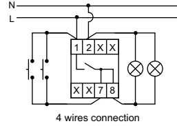
4 wires connection
