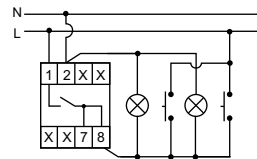
3 wires connection
