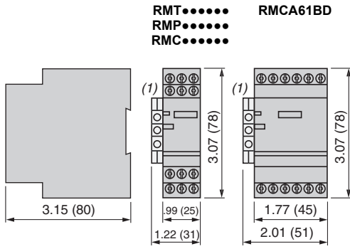
(1) Terminal block AB1 RRTP435U or AB1 RRTP435U2
