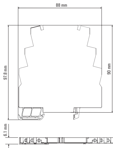
Screw connection
